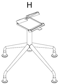
Flip-Top Arched X-Base
