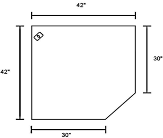
Corner Unit for 30" Left & 30" Right Connecting Units
